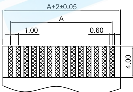
FFC/FPC Dimension Thickness:0.30±0.05 mm
